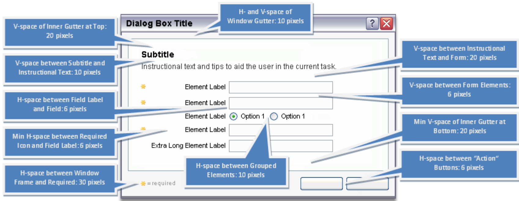
↑ Figure 21: Form Element Spacing in Dialogs
