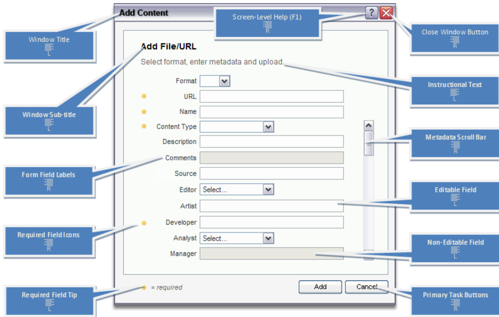
↑ Figure 11: Jumbo Dialog Box with Form
